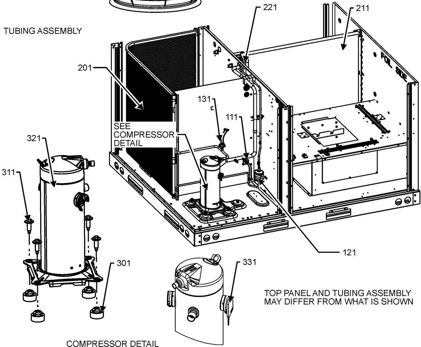
COMPRESSOR DETAIL
