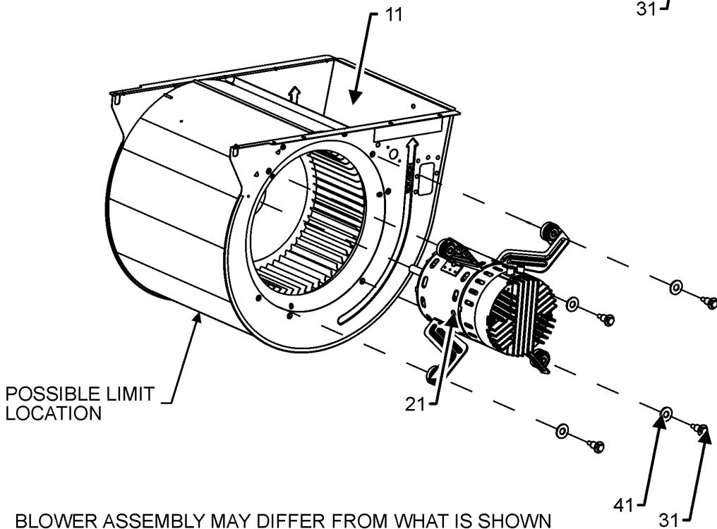
BLOWER ASSEMBLY 2
