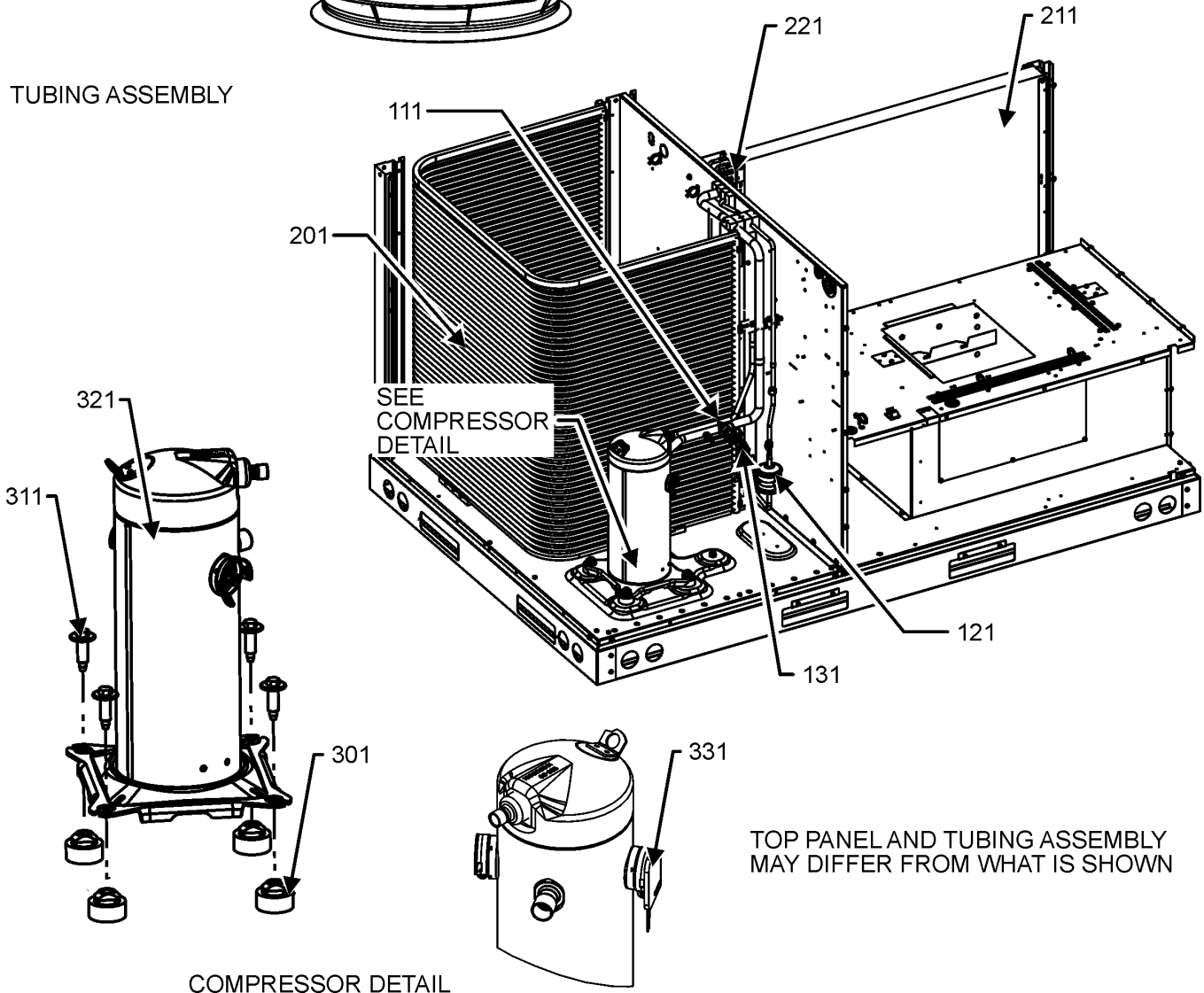
COMPRESSOR DETAIL
